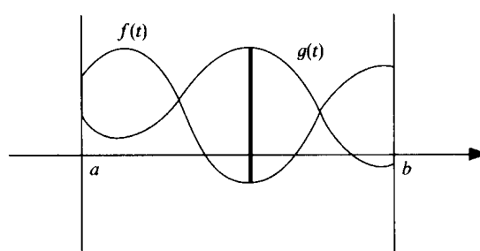
(b) d_\infty(f, g)
