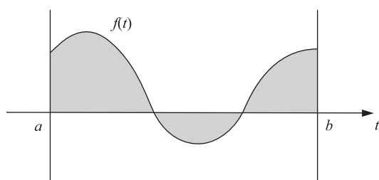
(a) \|f\|_1 is shaded.
