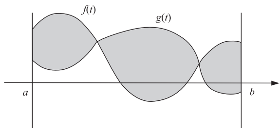
(b) d_1(f, g) is shaded.
